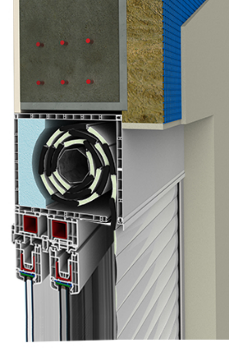
Monoblok Panjur
